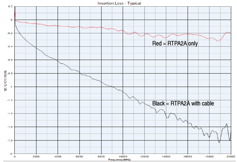
Figure 10: Insertion loss
