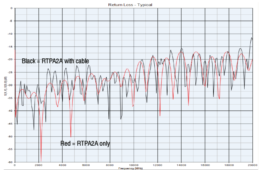
Figure 11: Return loss
